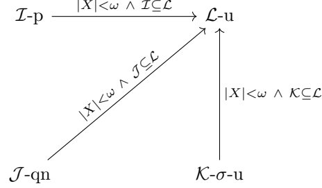
FIGURE 2. Diagram for Proposition 3.3, where “ \mathcal{I}\text{-p} \xrightarrow{|X| < \omega \wedge \mathcal{I} \subseteq \mathcal{L}} \mathcal{L}\text{-u} ” is a counterpart of the equivalence “(1) \iff (2)”, and similarly for other arrows.
